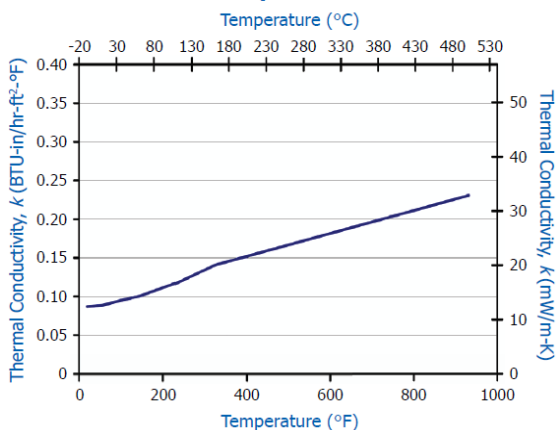
5 mm flexible blanket
